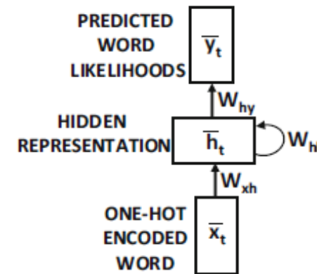
(a) RNN
